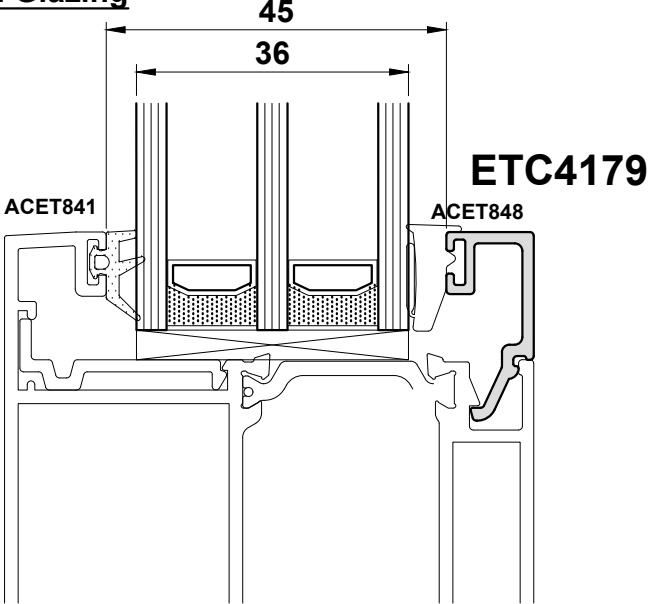
36mm Glazing
