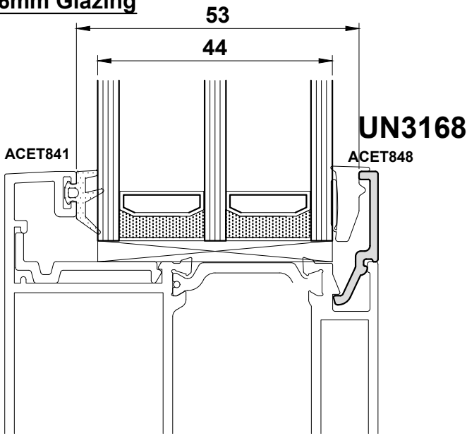
44-46mm Glazing
