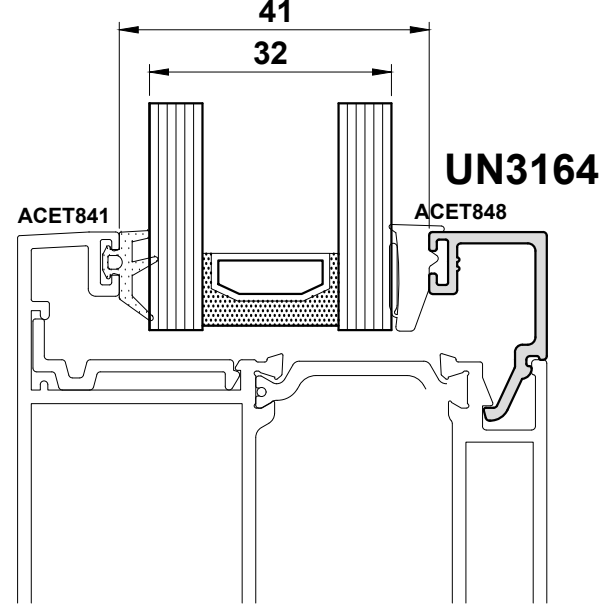
30-32mm Glazing
