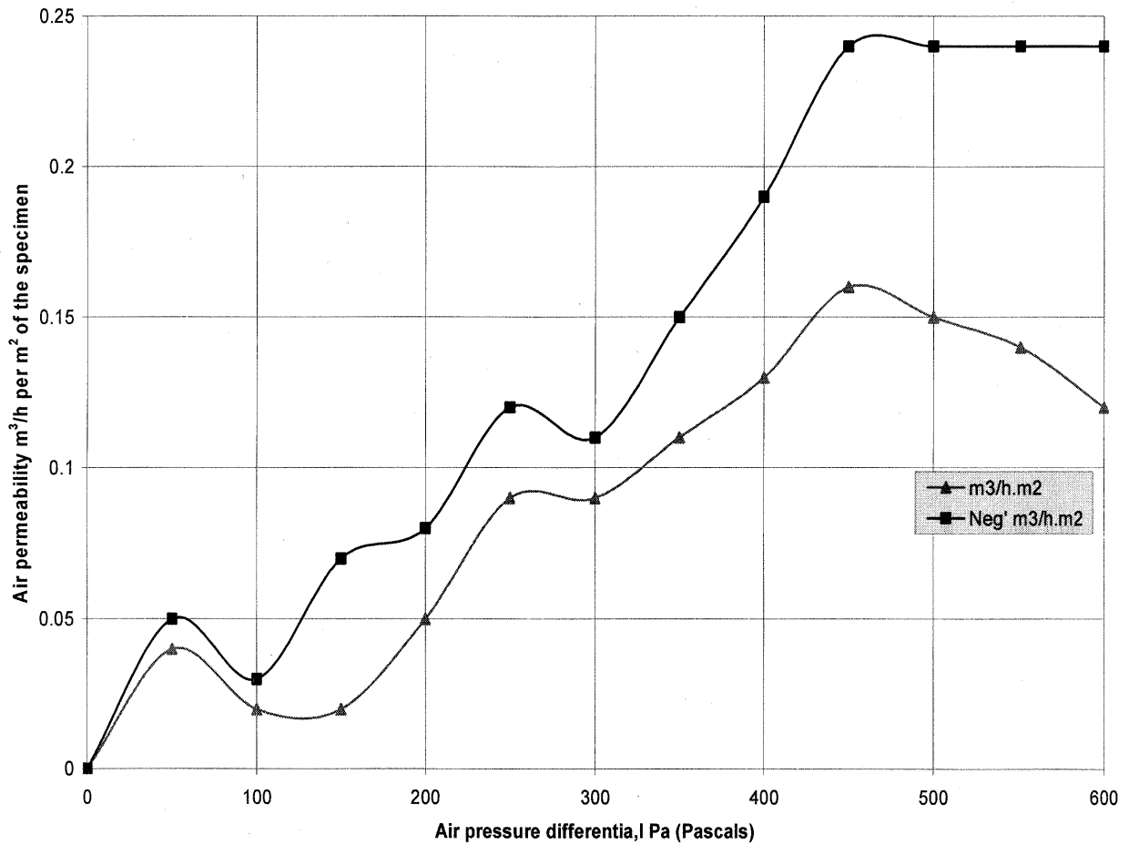
Figure A1. Air permeability under positive and negative air pressure; test results
