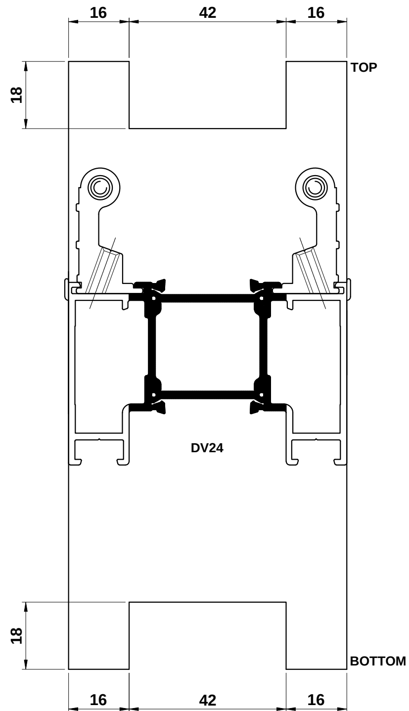
END MILLED
