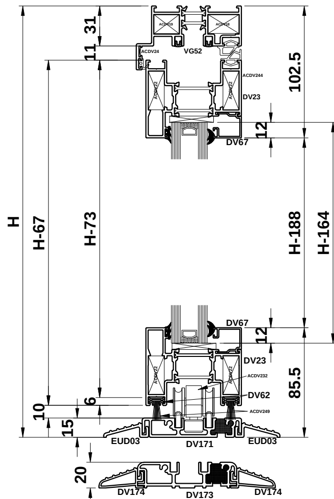
PROFILE CUTTING SCHEDULE (DV173)
