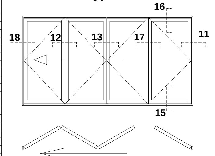
GLASS DEDUCTIONS
