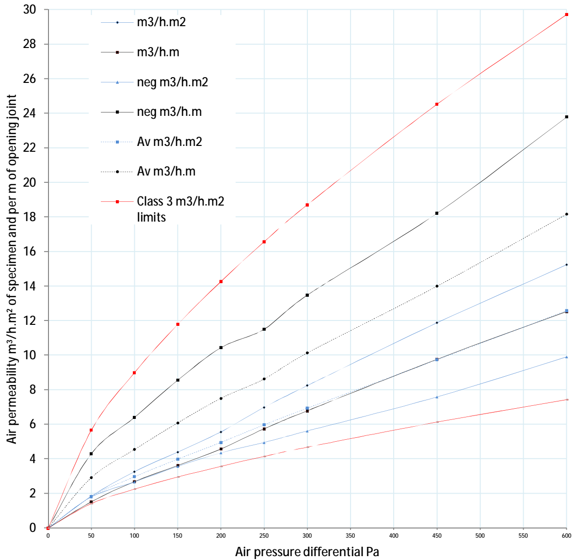
Figure A1. Test results: Air permeability under positive and negative air pressure; showing limits and averages of air permeabilities measured under positive and negative test pressures
